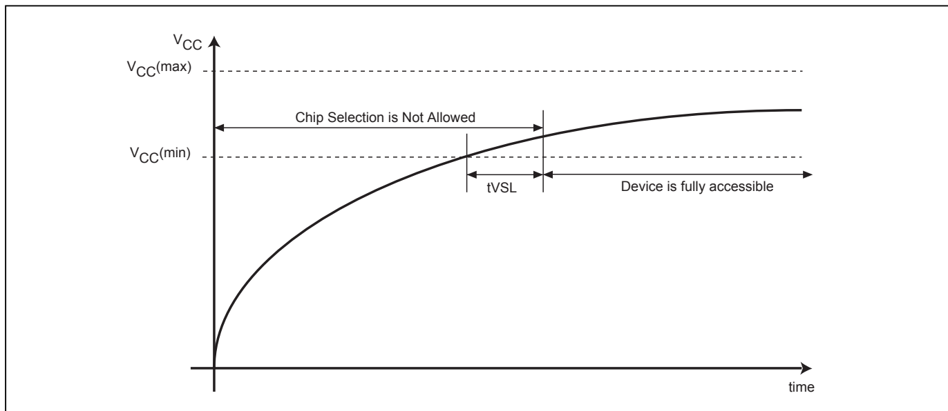
Figure 27. Power-up Timing
